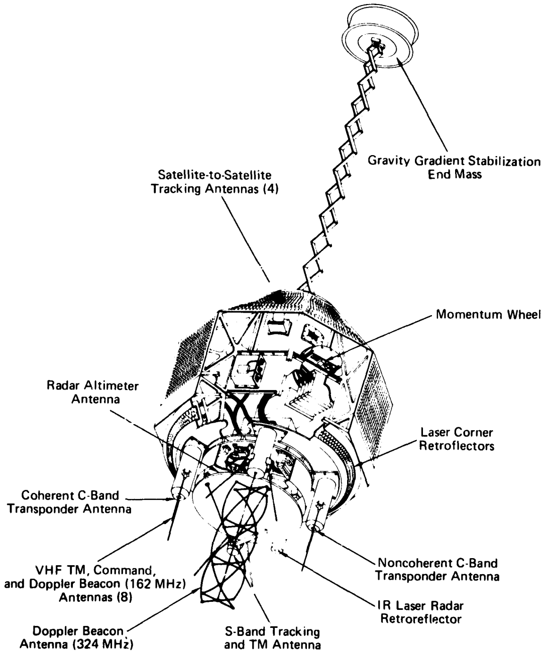
Fig. II-11 GEOS-C Cutaway View
