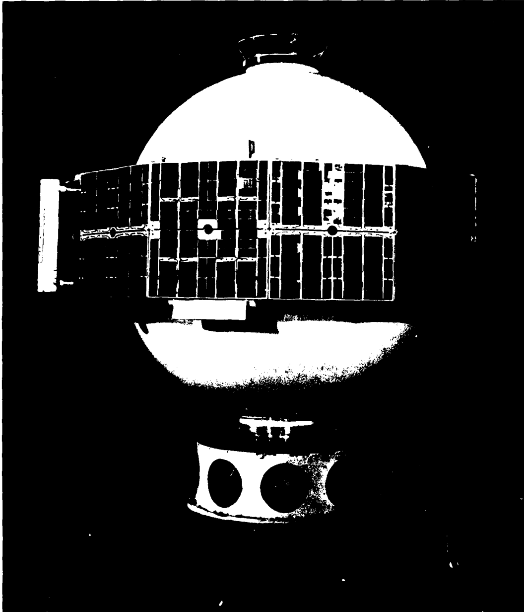
Fig. II-2 ANNA-1A Satellite
