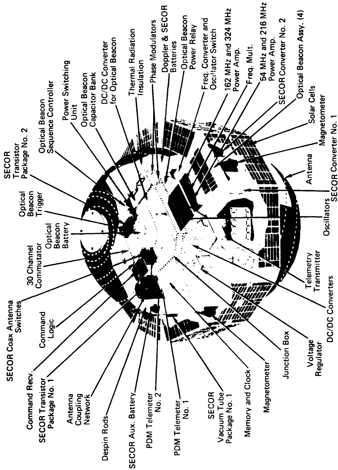
Fig. II-3 ANNA-1B Satellite, Cutaway View
